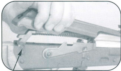
Spring loaded release button.
